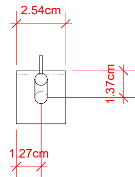
4 Vista Frontal Scale 1:2
