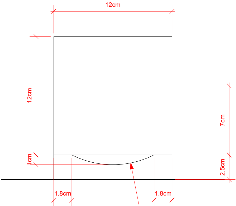
2 Scale 1:2 Vista Frontal
