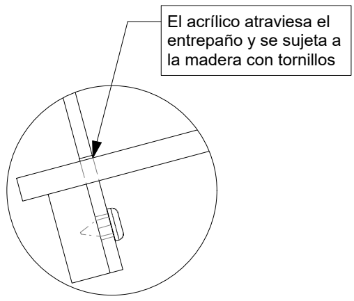
6 Vista Lateral Scale 1:2
