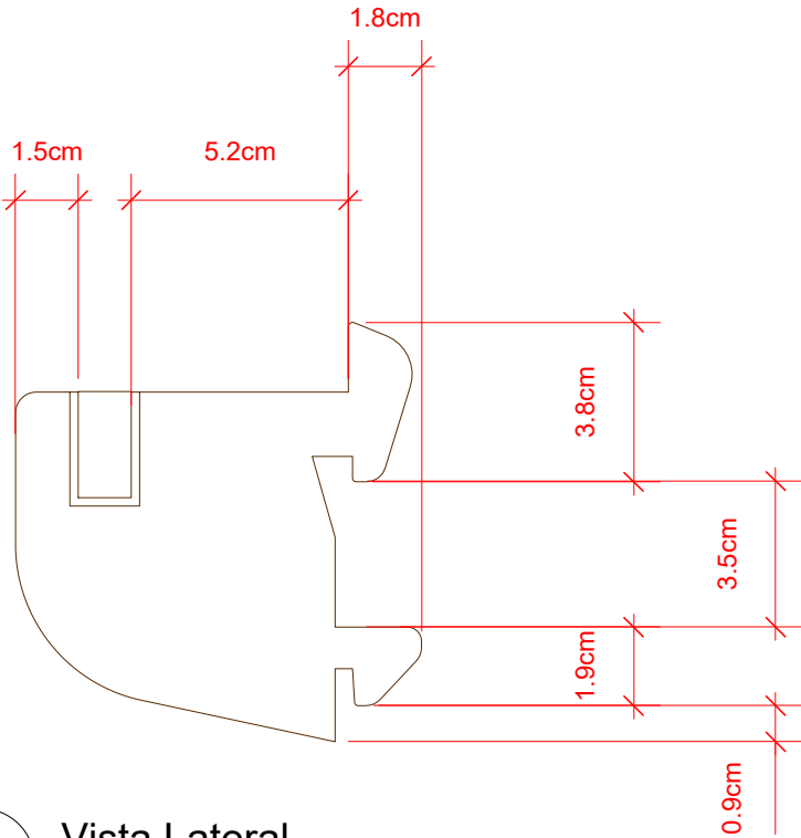
4 Vista Lateral Scale 1:2
