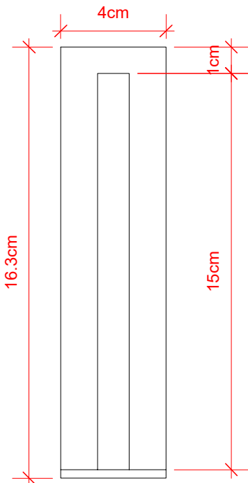
3 Vista Frontal Scale 1:2
