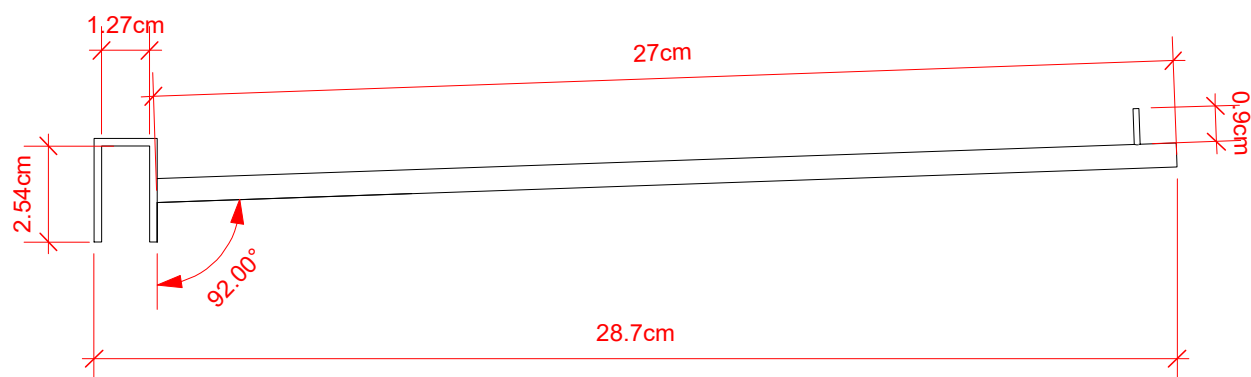
2 Vista Lateral Scale 1:2
