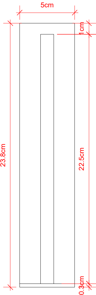
3 Vista Frontal Scale 1:2
