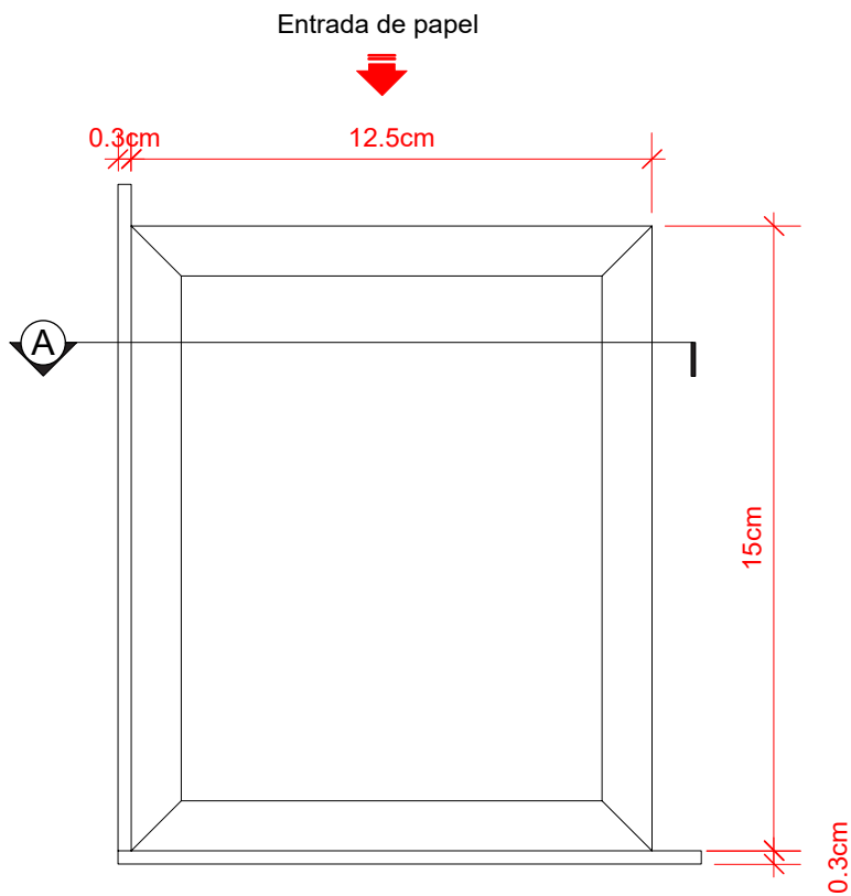
2 Vista Frontal Scale 1:2
