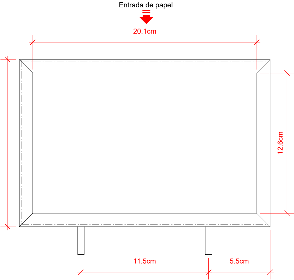
2 Vista Frontal Scale 1:2
