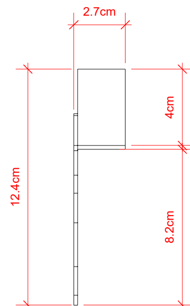
4 Vista Frontal Scale 1:2
